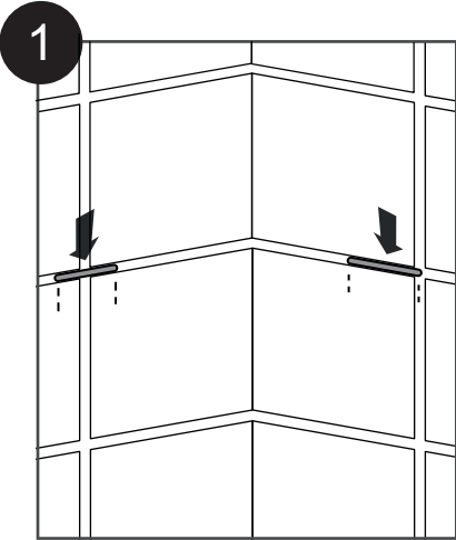
After completing tile installation, place 1/2" long spacers into install tab locations.
